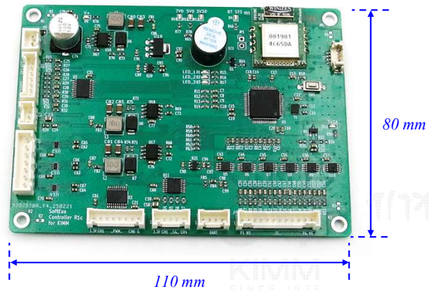
Main board
