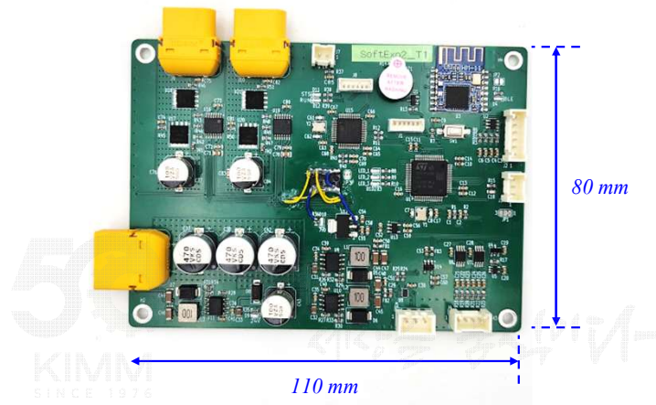
Main board + Current driver (2 ch)
