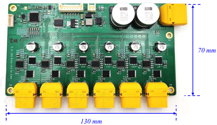
Current driver (6 ch)
